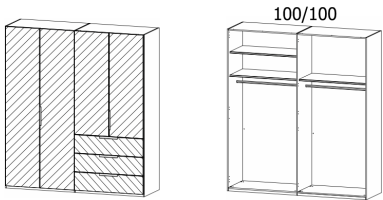
4 Doors, 3 Drawers W 201 X D 60 X H 223 cm
