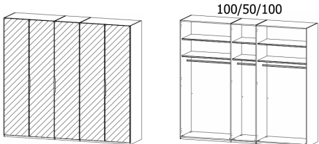
5 Doors W 251 X D 60 X H 223 cm
