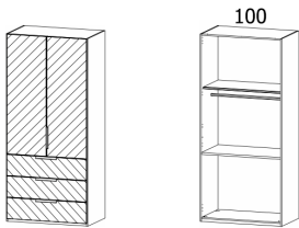
2 Doors, 3 Drawers W 101 X D 60 X H 223 cm
