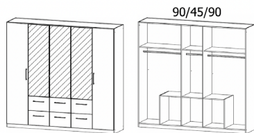
5 Door/6 Drawer Robe W 226 X D 54 X H 210 cm
