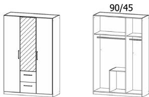
3 Door/2 Drawer robe W 136 X D 54 X H 210 cm
