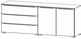
160cm 2 Door 3 Draw Chest W 160 X D 42 X H 61 cm
