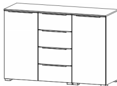
120cm 2 Door 4 Draw Chest W 120 X D 42 X H 81 cm
